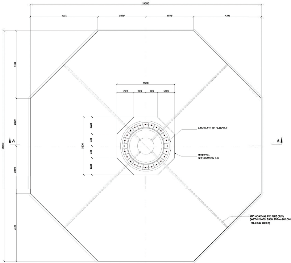
FOUNDATION LAYOUT
